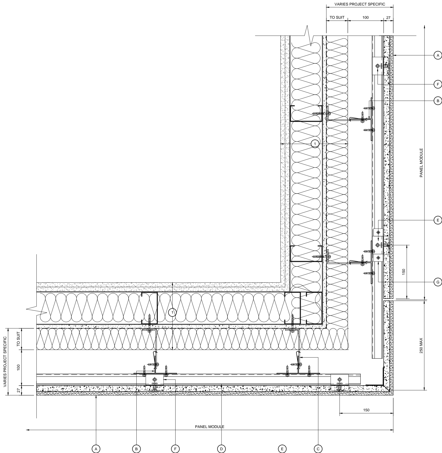
EXTERNAL CORNER DETAIL
